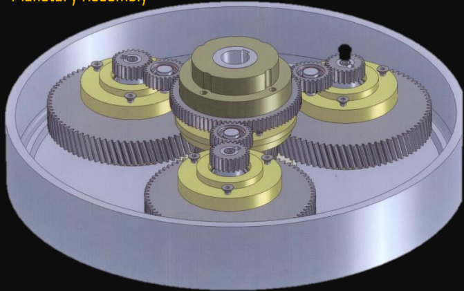
Interior of an Avenger's Planetary Assembly
